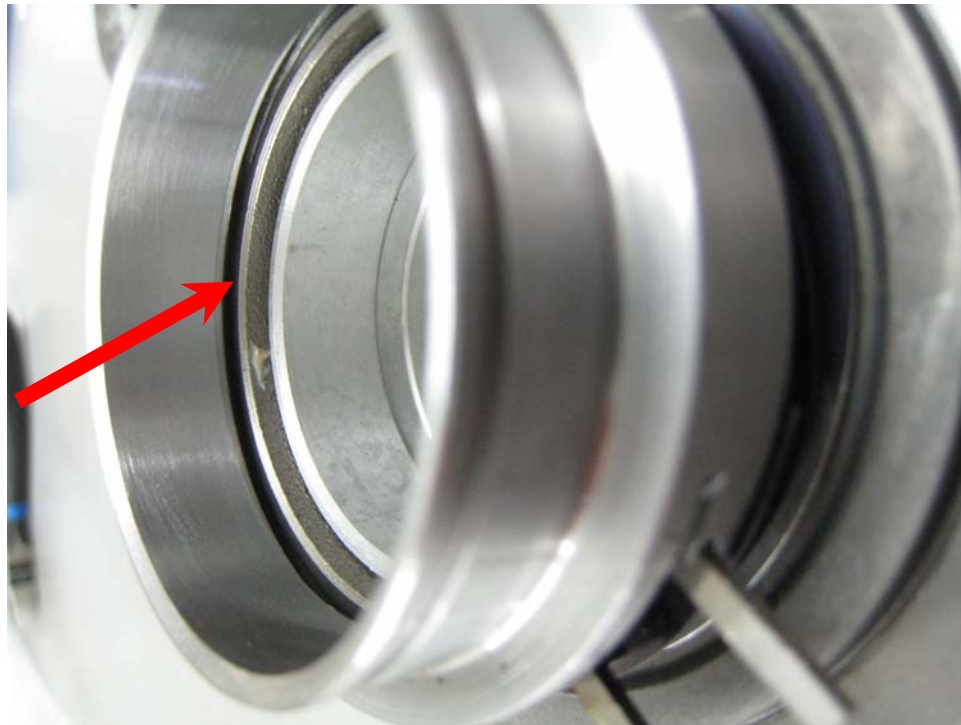
The internal groove for the Spiral ring is clearly visible between the adapter (closest to camera) and the Clutch Release Bearing.
